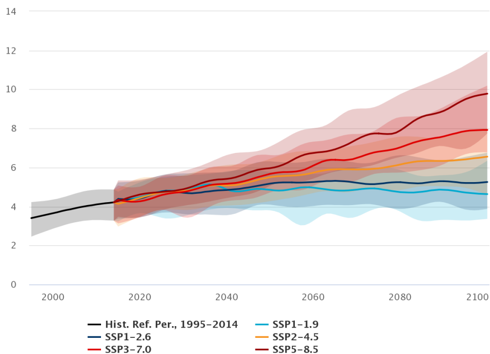
Projected Min-Temperature Zlatiborski, Serbia; (Ref. Period: 1995–2014), Multi-Model Ensemble
